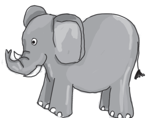
elephant
